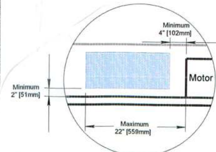
Electrical Conduit Location (Typical)
